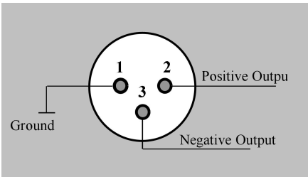
3-PIN XLR Male Connector
