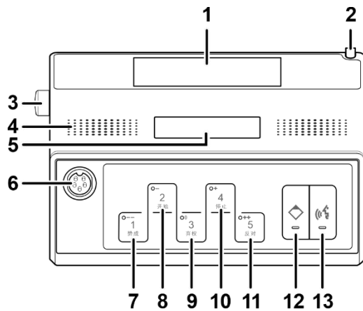
Top View of Chairman Unit
