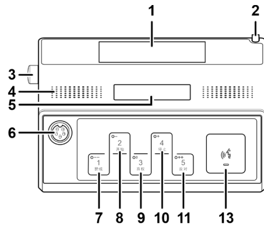
Top View of Delegate Unit
