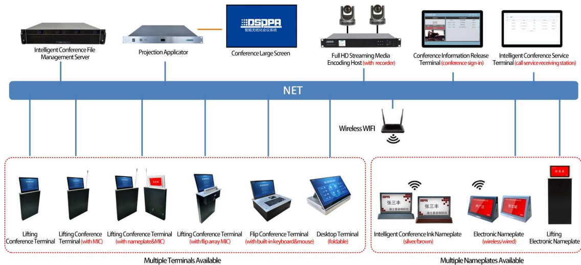
DSPPA Intelligent Paperless Conference System Topology
