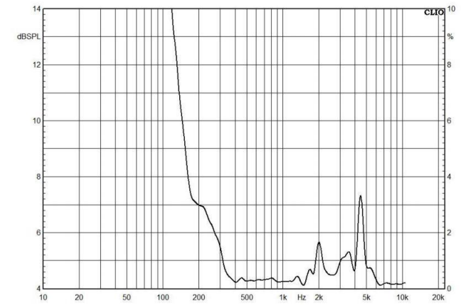
Distortion (THD<1.5% 1W,1m,100Hz-10KHz)
