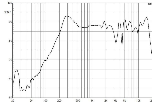
Freq.Response (dB SPL.1W.1m)
